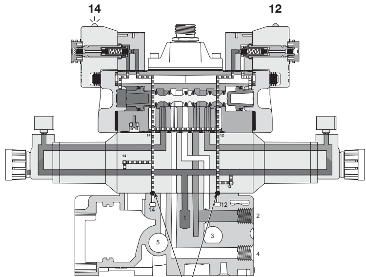
Sandwich Regulator has standard configuration of Internal Pilot with the Pilot Plug in the bottom #12 and #14 Pilot Hole which prevents line pressure from escaping through
