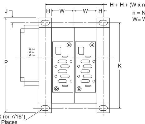
H2 - H3 Manifold Assembly
