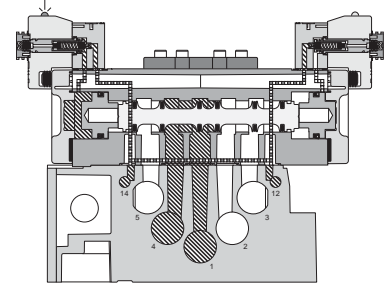
H3 5599-2 Double Solenoid External Pilot Subbase Mounted
