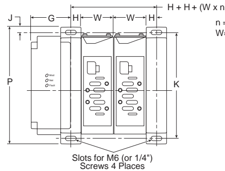
H1 Manifold Assembly
