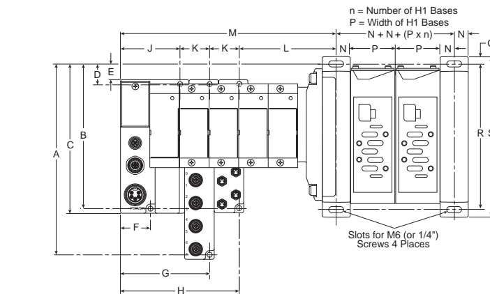
H1 Manifold Assembly
