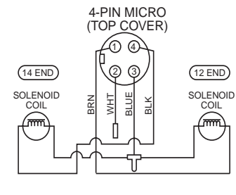
4-Pin Male / Double Solenoid (Encl. Option 2, Auto Option G)
