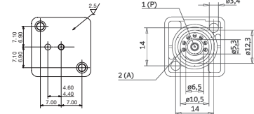
Operator mounting pattern (mm)
