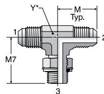
Y* – Across wrench flats
