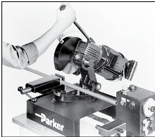
Fig. S11 – Cut-off Saw on Parker's TP432 or TP1025 Tube Preparation Center
