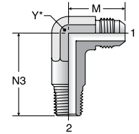
Y* – Across wrench flats
