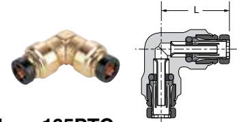
Tube to Tube Union Elbow 165PTC
