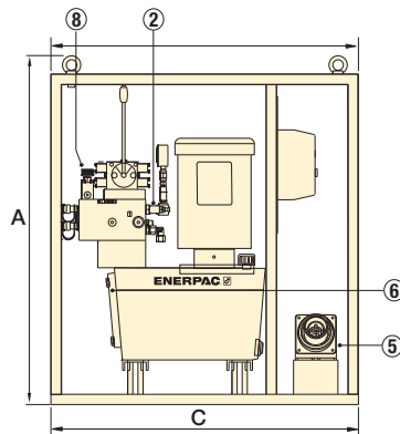
◀ SFP-Series with 10 gallon reservoir (shown with 4 split-flow outlets)
