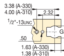
Top View Working Surface
