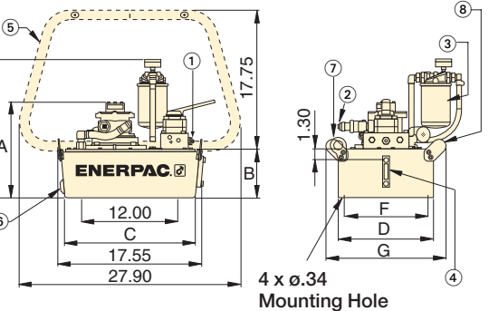
2.5, 5, 10 gallon reservoirs
